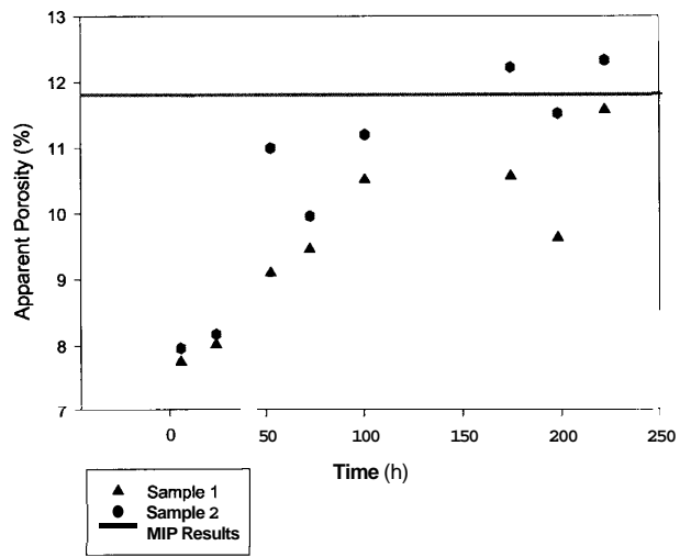
Figure 2 Porosity measurements of partially stabilized zirconia samples.
