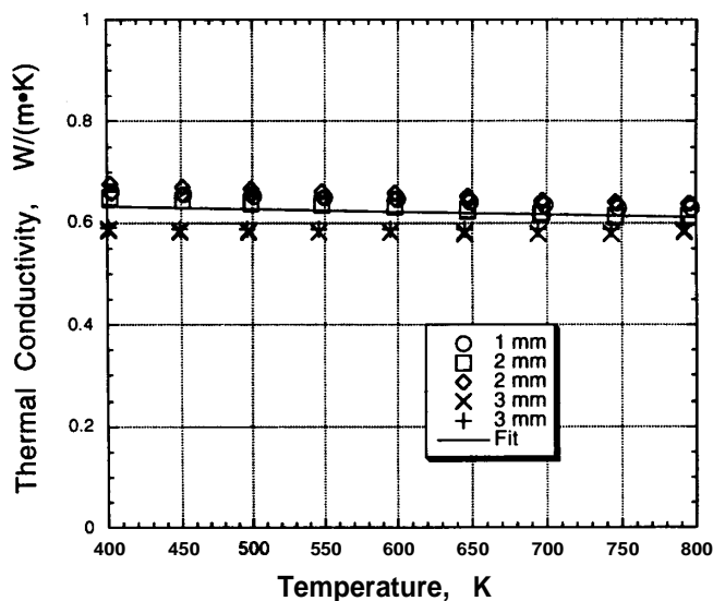
Fig. 6 Thermal conductivity of an atmospheric plasma-sprayed 8YSZ coating
