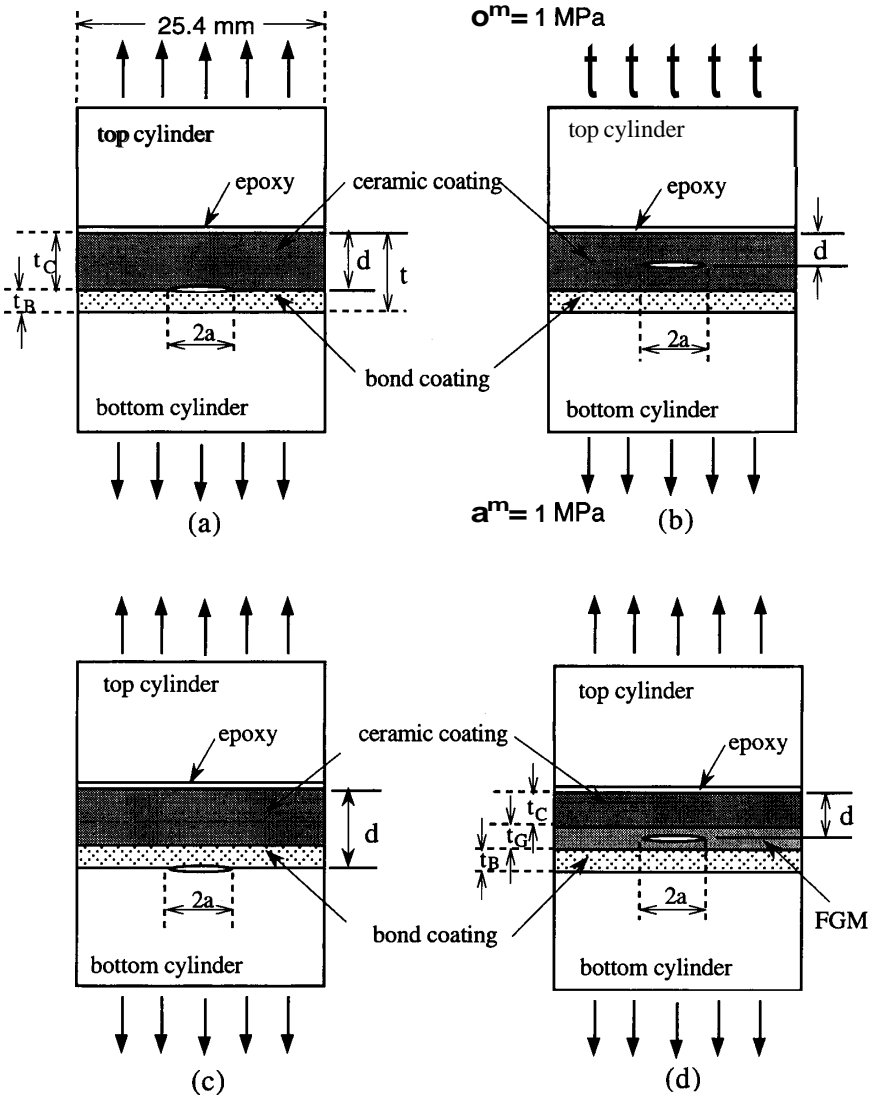
Fig. 2. Various locations of initial embedded cracks shown in the cross-sections of axisymmetric models. Tensile loading is assumed to be \sigma^x = 1 \text{ MPa} . The coating thickness, the crack size and the cylinder diameter are not drawn in scale. (a) Interface crack between the ceramic and bond coatings. (b) Homogeneous crack within the ceramic coating. (c) Interface crack between the bond coating and the substrate (bottom cylinder). (d) Crack in the functionally graded material.
