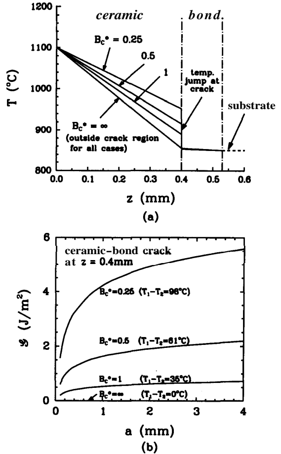
Fig. 11. (a) Temperature profile inside the crack region of the ceramic–bond interface crack model. The effective Biot numbers B_c^* are noted for different temperature jumps across the crack surfaces. For each case, the temperature profile outside the crack region is always given by the B_c^* = \infty profile. (b) Energy release rate as a function of embedded crack radius for different temperature jumps across the crack surfaces. The result for B_c^* = \infty (no temperature jump) is extremely small.
