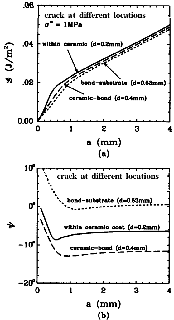
Fig. 4. (a) Energy release rate as a function of embedded crack radius for cracks at different locations. The specimens are under tensile pressure of 1 MPa. (b) Corresponding phase angle.
