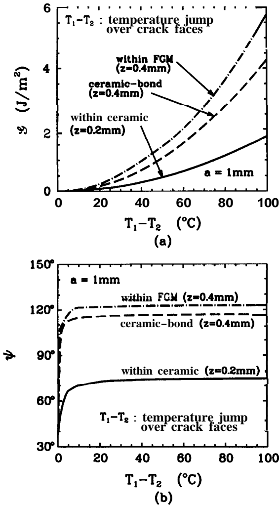
Fig. 14. (a) Energy release rate as a function of temperature jump across the crack faces. The results are shown for cracks at various locations. In all cases, the radius is a = 1 mm. (b) Corresponding phase angle.
