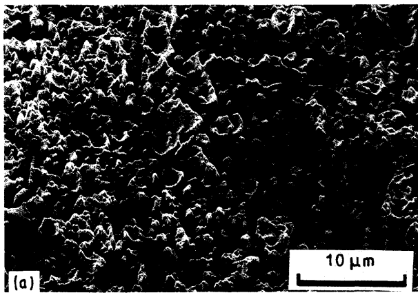
Figure 7 Surface of WC-12% Co FARE gun comb: (a) unused; (b) after 10 min wear test.
