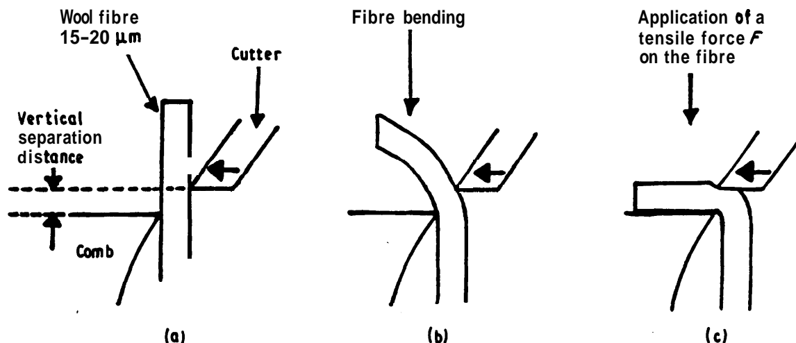
Figure 9 Incorrect adjustment of comb and cutter pair. (a) Vertical separation between comb and cutter. (b) Fibre bending as cutter advances. (c) Fibre bent at right angles between cutter and comb.
