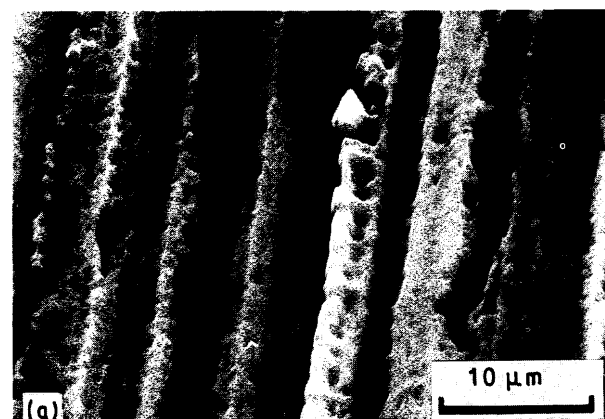
Figure 4 Surface of TiN-coated comb: (a) unused; (b) after being used in a field trial on 100 sheep.
