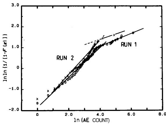
Figure 11 Weibull plot for acoustic emission count data of specimen 2 for two different thermal cycles.
