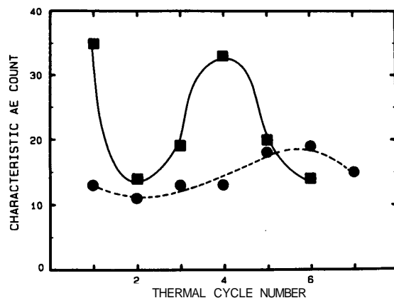
Figure 12 The characteristic acoustic emission count of plasma sprayed coatings subjected to thermal cycling. (■ specimen 1, ● specimen 2).
