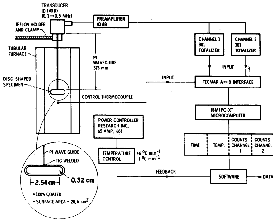
Figure 3 Schematic of experimental arrangement.
