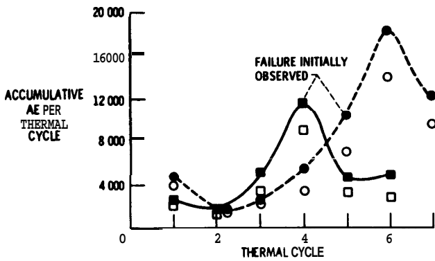
Figure 5 Accumulative AE per thermal cycle for two ceramic coatings. □ ■ thick (5.19 g ceramic). ○ ● thin (3.97 g ceramic). ● ● Channel 1, 91 dB (x 35480). □ ○ channel 2 88 dB (x 25 120).
