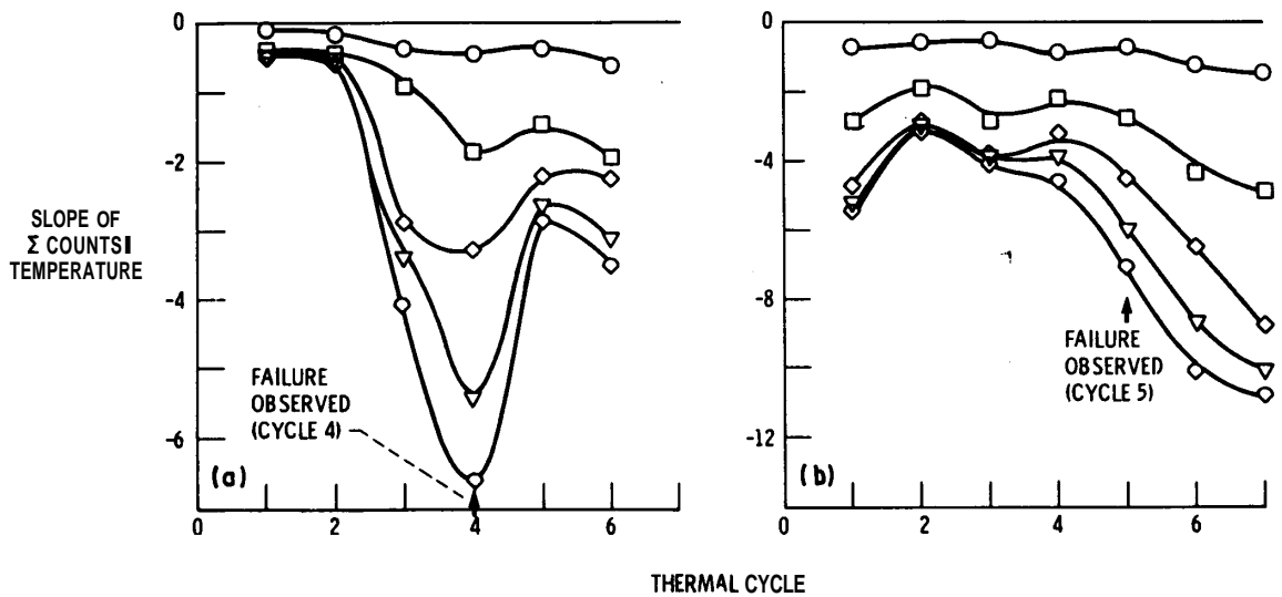
Figure 7 Influence of the bound level and thermal cycle number on the gradient of the accumulative count plotted against temperature data. (a) specimen I, (b) specimen 2, (bound level in counts per event: ○ 10, □ 30, ◇ 50, ▽ 70, ○ 90).
