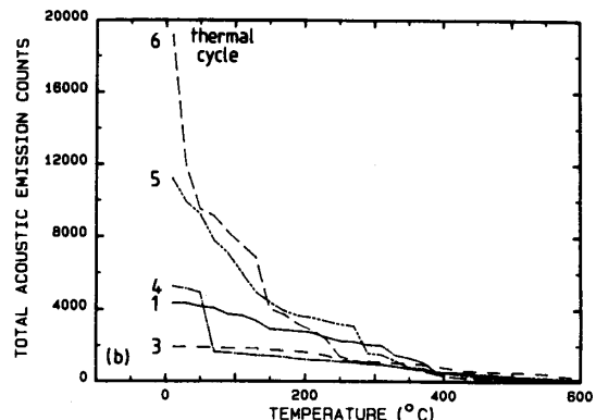
Figure 6 Accumulative counts plotted against temperature data. (a) specimen I. (b) specimen 2.
