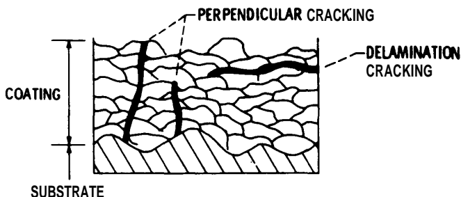
Figure I Schematic of crack morphologies in plasma sprayed coatings.
